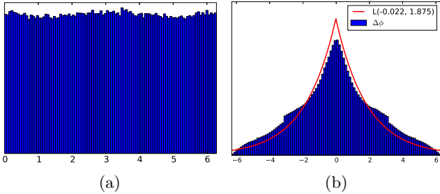
Figure 4: The mean distribution of \Delta\phi of the BraTS simulated images. The images were registered using a rigid transformation and only the tumour areas were sampled. (a) the distribution of \Delta\phi in the simulated tumour region. (b) the distribution of \Delta\phi over the entire image. It also shows the Laplacian distribution that best fits the data.
