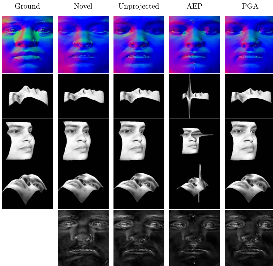
Figure 4.10: The reconstructions of subject srb. The first row is the normal map. The second row is a profile rendering. The third row is a side view. The fourth row is a rendering from below the chin. The final row is the angular error between the reconstruction and the ground truth.
