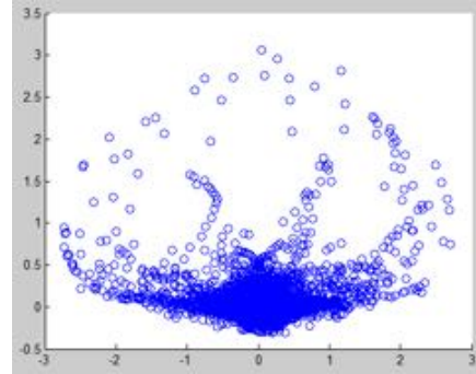
Projection to the tangent plane at the mean point.
